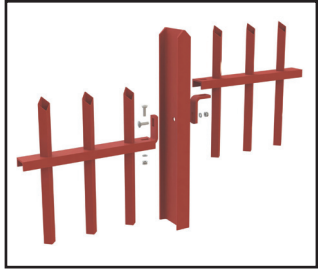
Special angle cleats allow panels to be stepped. 0-35mm & 85-123mm on site
